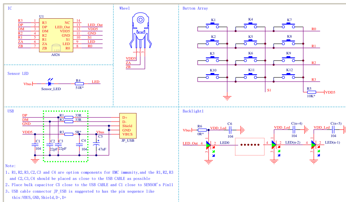
Figure 3. Application circuit with specialized LED
