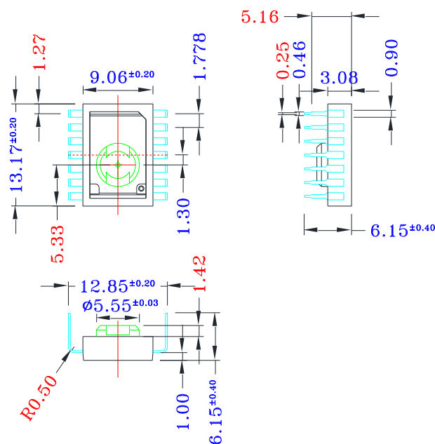
Figure 5. Package Outline Drawing
