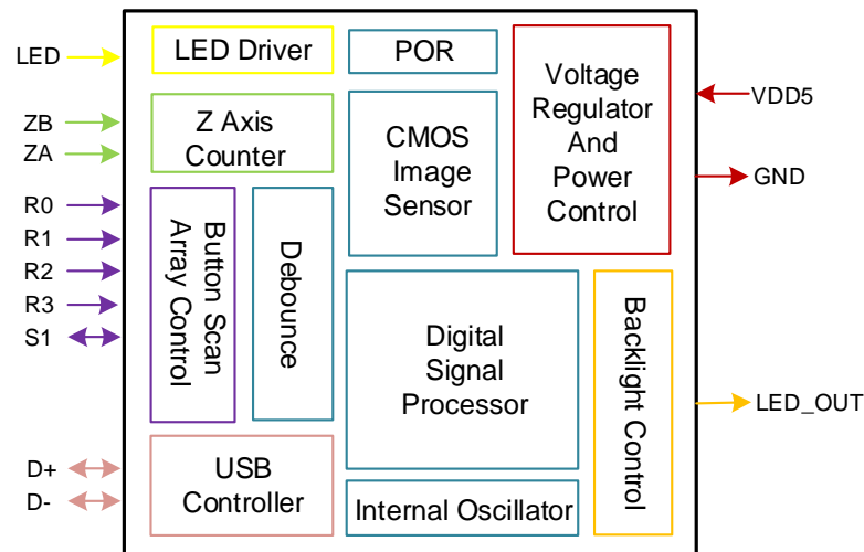
Figure 2. Block Diagram
