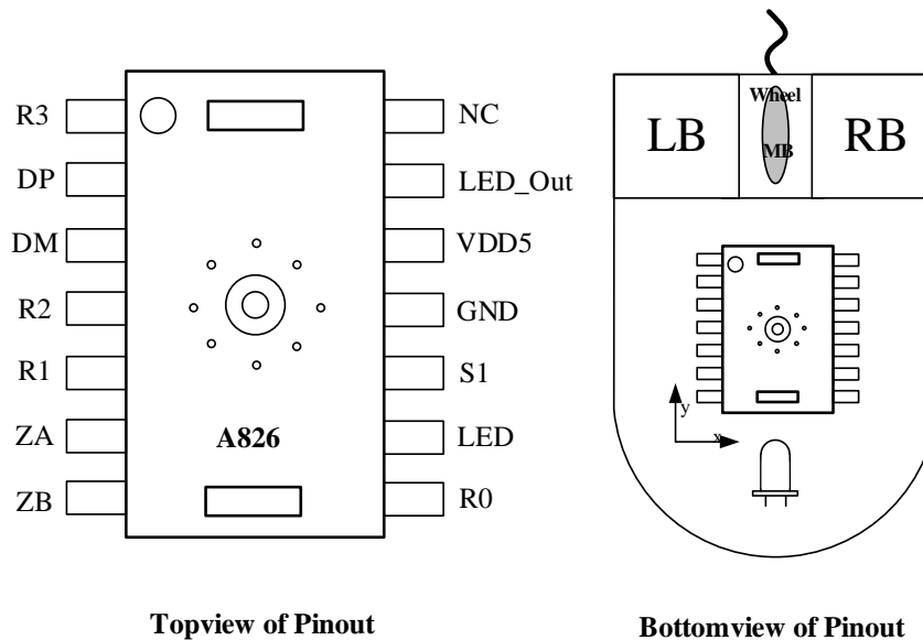
Figure 1. Pinout
