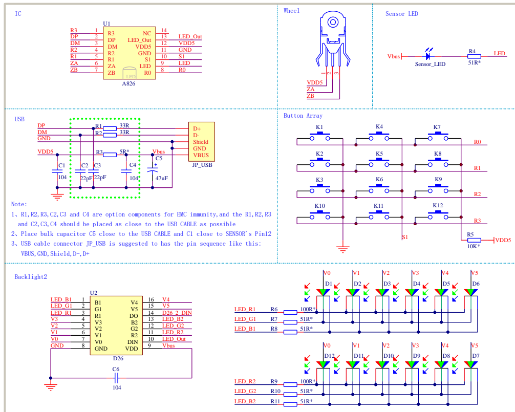
Figure 4. Application circuit with D26
