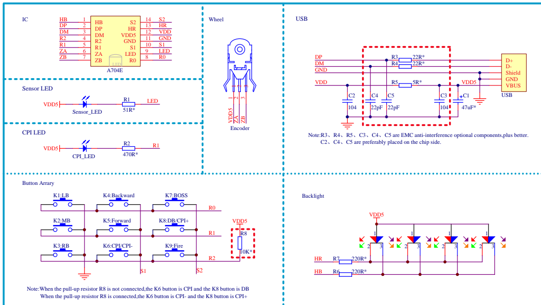
Figure 3. Application Circuit
