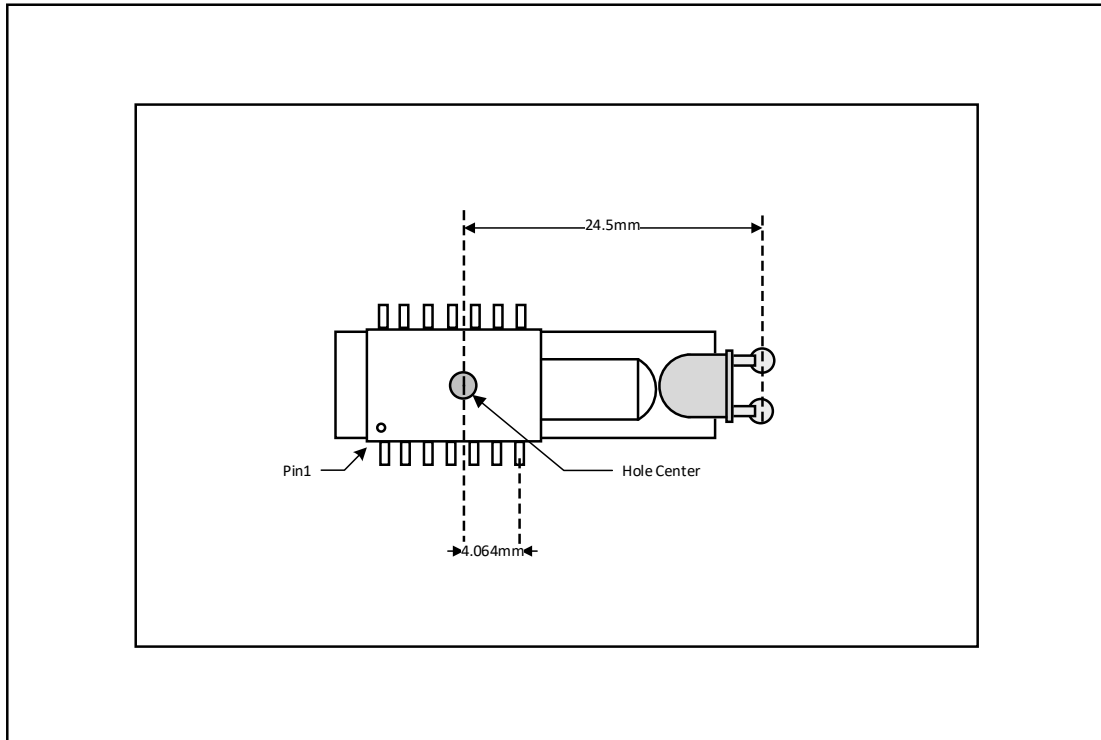
Figure 5. 2D Assembly drawing of A704E (Top and Side View)
