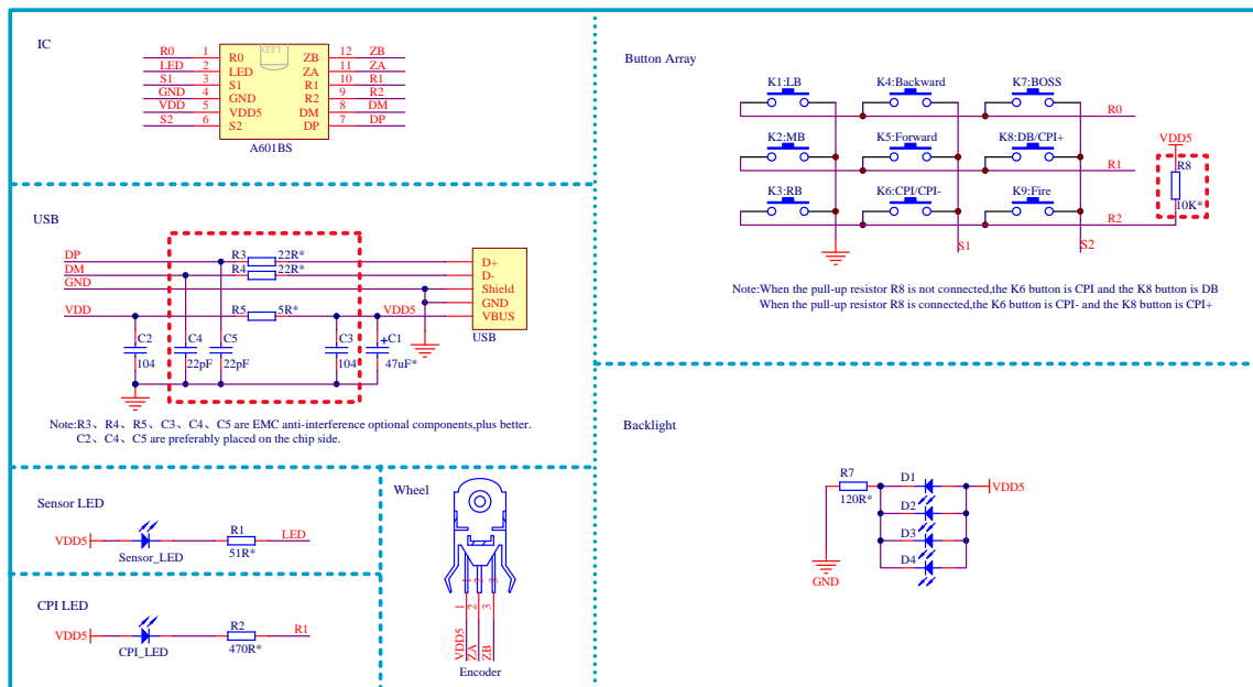
Figure 3. Application Circuit
