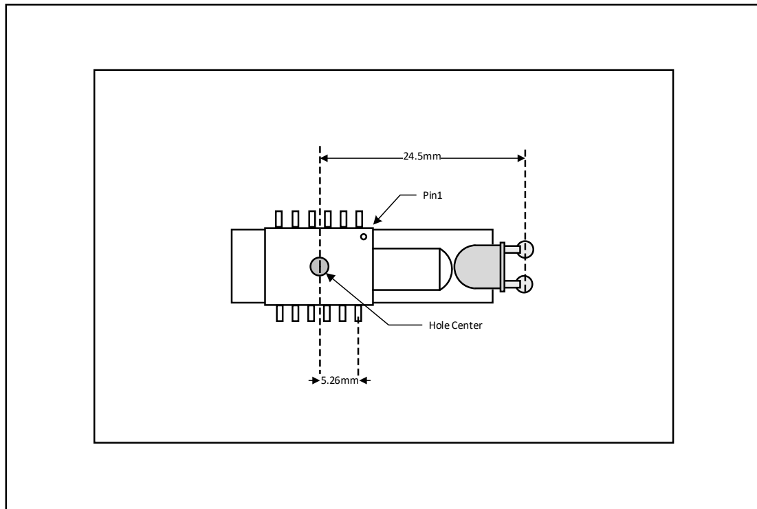
Figure 5. 2D Assembly drawing of A601BS (Top and Side View)
