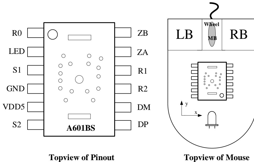
Figure 1. Pinout
